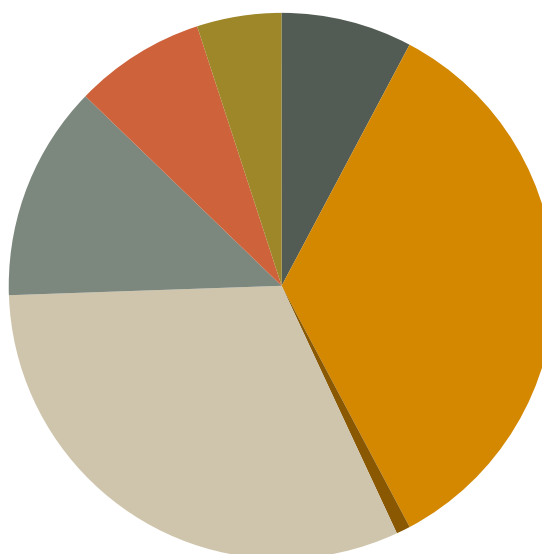
January 2010
