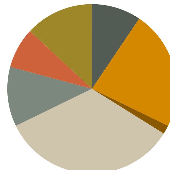
May 2010
