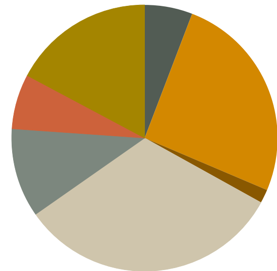
May 2010
