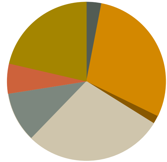
May 2010
